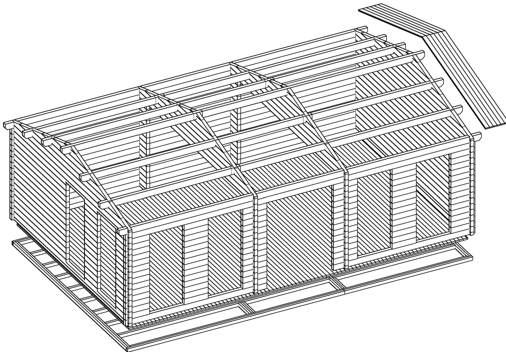
HansaGardenRoom70D ISO
